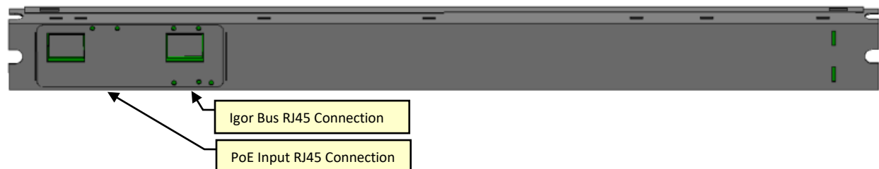
Figure 2 – Linear Network Node Bottom
