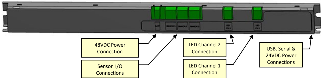
Figure 2 – Linear Network Node Bottom
